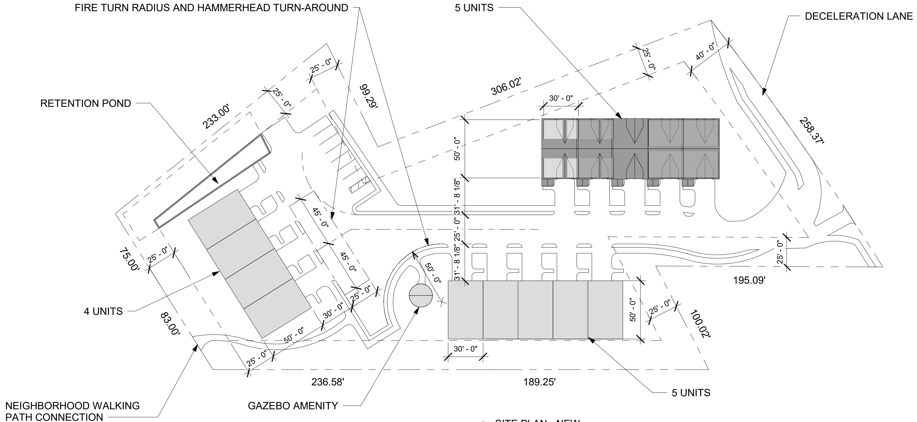
① SITE PLAN - NEW 1" = 50'-0"
